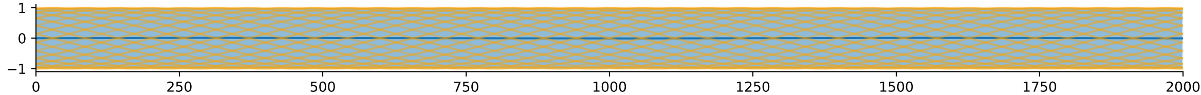
Output Tensor
