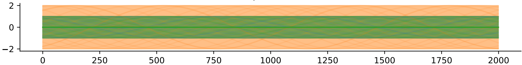
Output Tensor
