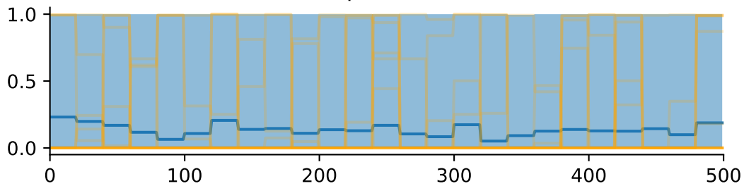
Output Tensor
