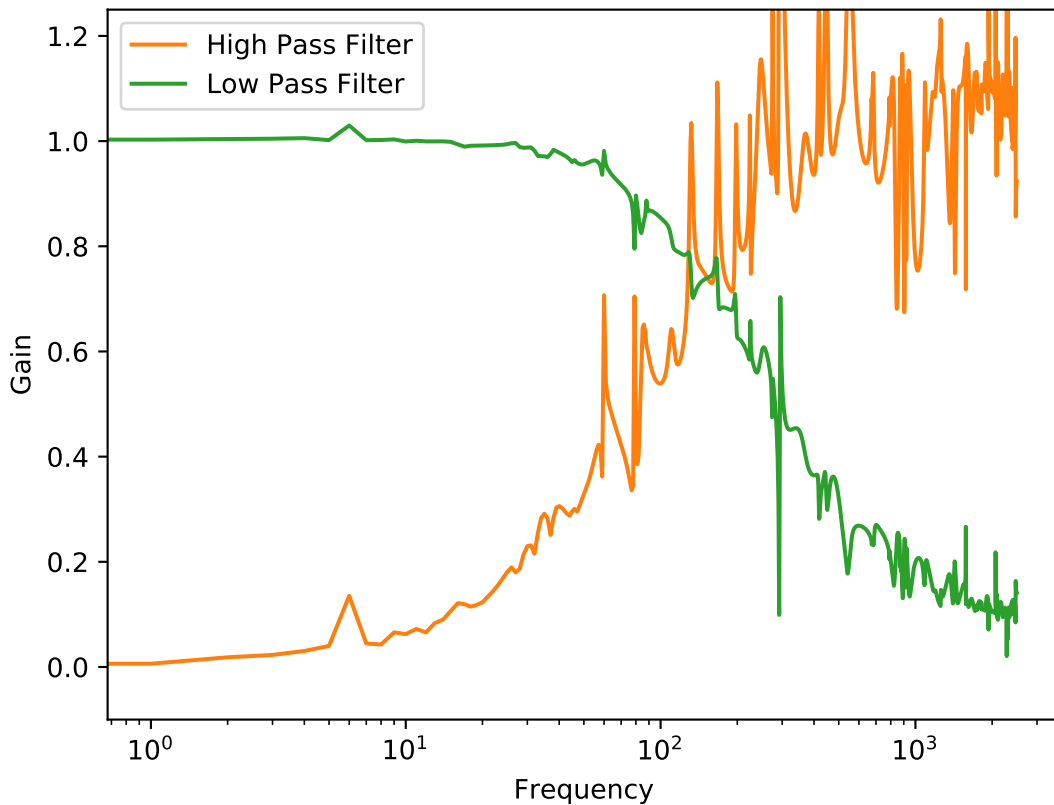
Transfer Functions of Filters
